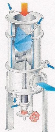
Venturi Quench System REITHER
