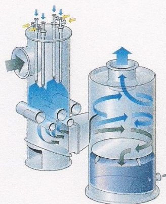
Venturi Scrubber System BAYER-REITHER
