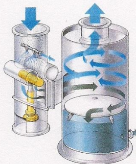
Venturi Scrubber System REITHER
